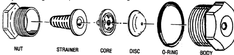
L-W Nozlet Full Cone Spray Nozzle (1 1/16" NPT pipe thread)
